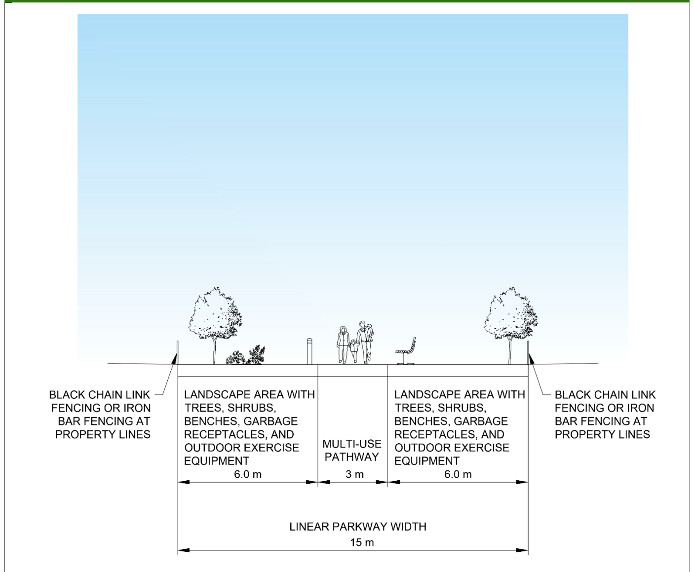
Figure 6-1 Linear Park Cross Section
