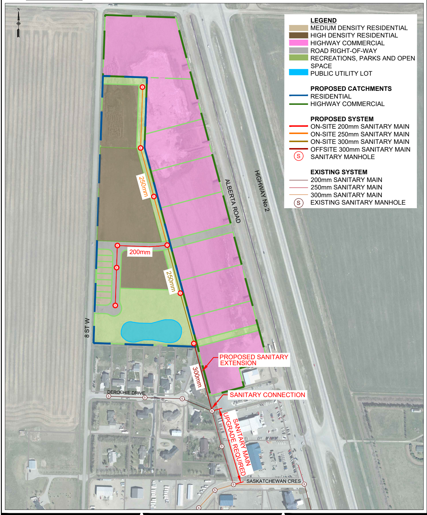
FIG 6-5 - SANITARY SYSTEM
